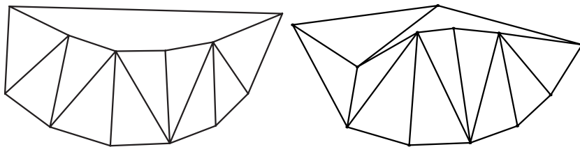
FIGURE 6. A Laman circuit and one of its embeddings as a pseudo-triangulation with exactly one non-pointed vertex.
