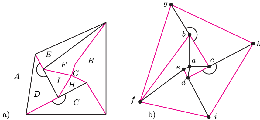
FIGURE 9. We can have flat angles on both sides of a non-crossing reciprocal pair.
