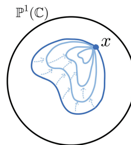
Figure 1. Any loop is retracted on \mathbb{P}^1(\mathbb{C}) .
