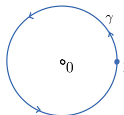
Figure 2. A nontrivial loop \gamma on \mathbb{P}^1(\mathbb{C}) \setminus \{0, \infty\} .
