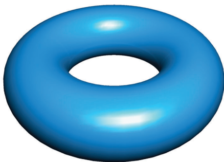
Figure 3. Riemann surface of genus g = 1 .
