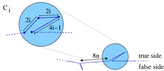
Figure 1: The chain encoding the configuration
