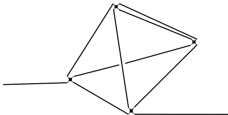
Figure 13: A polygonal chain forming a rigid tetrahedron \tau
