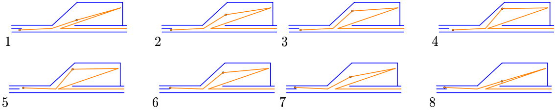
Figure 3: Animation showing how the chain can move around the notch when the checked variable has the right value
