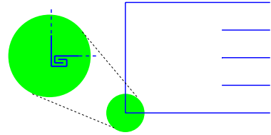
Figure 12: Making the environment-tree rigid
