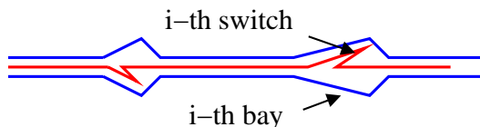
Figure 9: Setter allowing the i -th bit (among others) to flip
