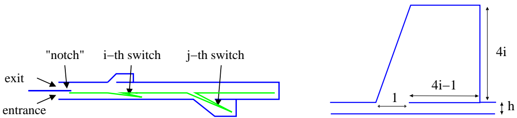
Figure 4: Checking the 2-clause (z_i \vee \bar{z}_j)
