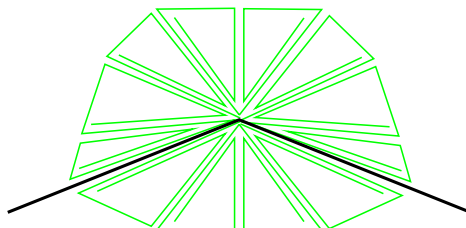
Figure 2: Fixing a hinge
