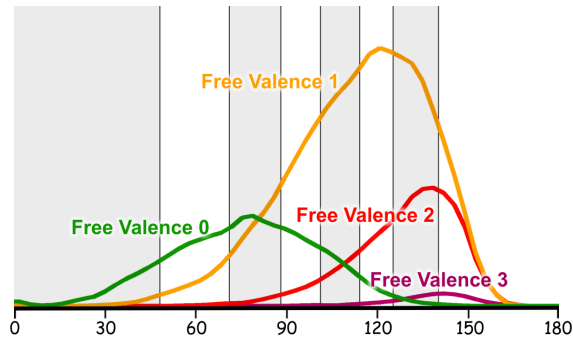
Figure 5: Distribution of opening angles for an encoding run of the Max Planck model. Each free valence has its own distribution. Note how the curves for different values of free valences overlap due to the irregularity of the mesh. Negative opening angles can occur at vertices with negative Gauß curvature and at boundary vertices. The vertical gray and white bars show the optimized thresholds by which FreeLence groups symbols into contexts.
