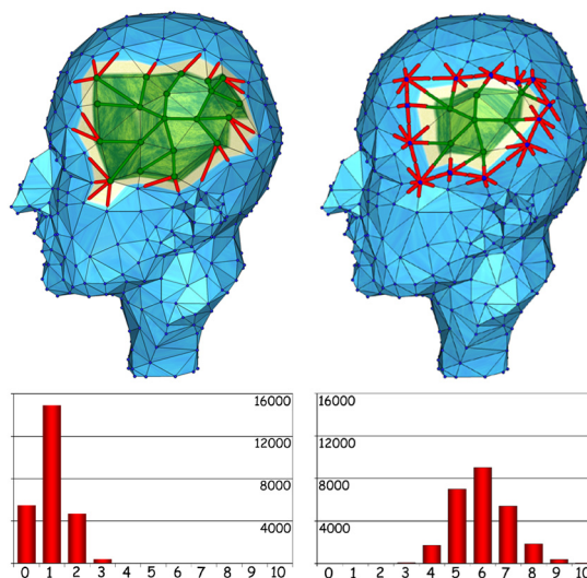
Figure 1: Geometry-driven coding with free valences (left) will in practice yield a lower symbol dispersion than coding with full valences (right). The frequency of local splits ( N and P ) as well as global splits is negligibly low for this particular model.
