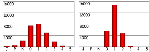
Figure 4: Symbol frequencies of free-valence codes of the Max Planck model for a simple spiraling mesh traversal (left) vs. FreeLence’s geometry-driven traversal (right). Local splits are denoted by P (previous) and N (next), global splits by J (join).
