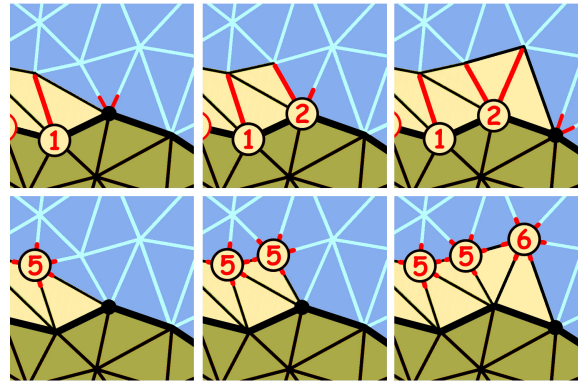
Figure 2: Encoding with free valences (top) versus encoding with full valences (bottom).
