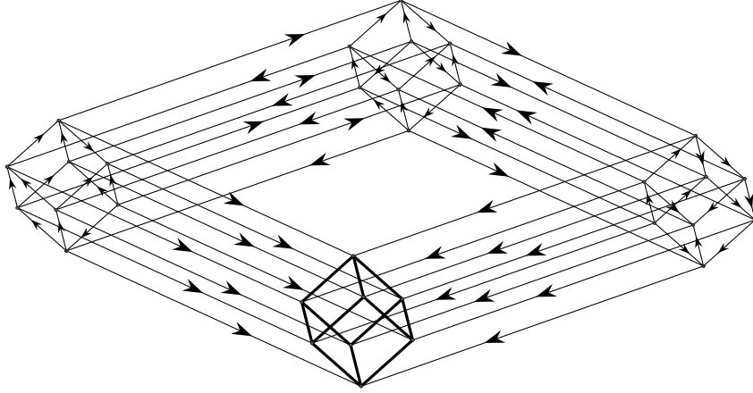
Figure 2: Three-dimensional flippable subcube
