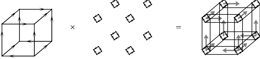
Figure 1: A product of a three-dimensional USO with two-dimensional ones
