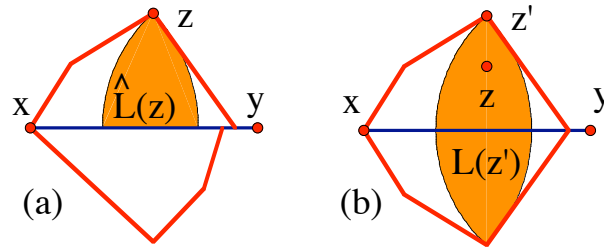
Figure 4: Figure (a) shows a half-lens in non-symmetric adornment, and Figure (b) show a symmetric lens with a point z in the interior of the lens and the adornment.
