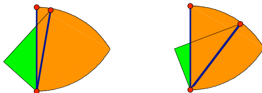
Figure 13: This is an example of two chains with non-symmetric slender adornments, where the expanded chain with adornments has smaller area.
