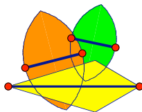
Figure 12: This Figure shows three intervals with overlapping symmetric slender adornments.
