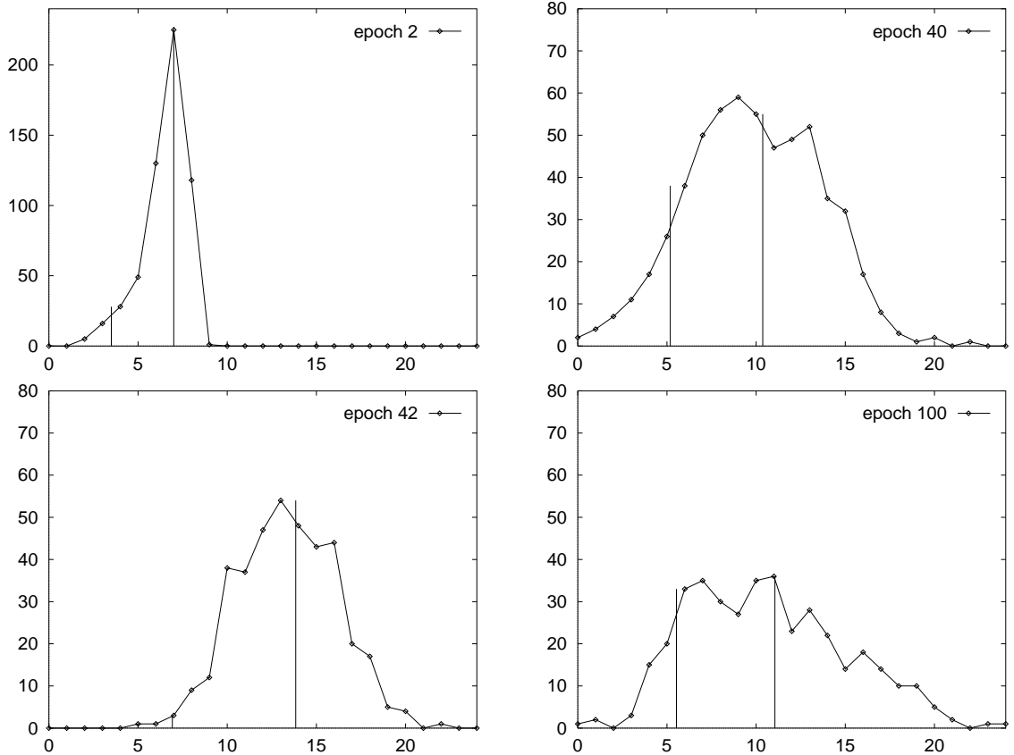
Figure 1: Four pruning coefficient histograms from the same training run (glass1 problem with pivot architecture) in epochs 2, 40, 42, and 100. Horizontal axis: coefficient size, grouped in classes of width 1. Vertical axis: absolute frequency of weights with this coefficient size. The right vertical line is the arithmetic mean of the coefficient sizes, the left vertical line is 0.5 times that. The area under the curve left of the left line thus indicates what would be pruned at that point for \lambda = 0.5 when a pruning step would occur. In the run shown, pruning occurred after epoch 40.
