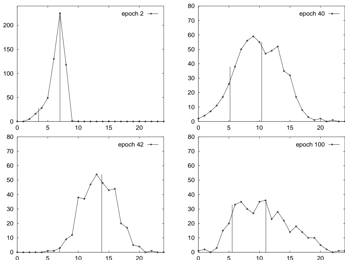
Figure 1: Four pruning coefficient histograms from the same training run (glass1 problem with standard architecture) in epochs 2, 40, 42, and 100. Horizontal axis: coefficient size, grouped in classes of width 1. Vertical axis: absolute frequency of weights with this coefficient size. The right vertical line is the arithmetic mean of the coefficient sizes, the left vertical line is 0.5 times that. The area under the curve left of the left line thus indicates what would be pruned at that point for \lambda = 0.5 when a pruning step would occur. In the run shown, pruning occurred after epoch 40.
