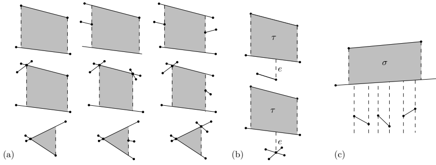
Fig. 3 (a) A trapezoid is defined by 2,3 or 4 line segments. (b) The handle e of a racquet (\tau, e) is defined by 1 or 2 segments. (c) In an opaque representation, the trapezoid \sigma is incident to 4 vertices, in a planar graph representation, it is incident to 10 vertices.
