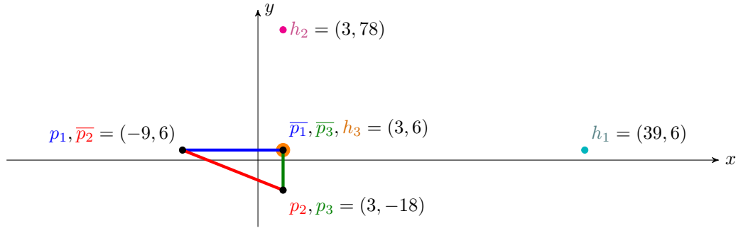
■ Figure 2 Construction of the point sets corresponding to the M2SAT instance (x_1 \vee \bar{x}_2) \wedge (x_2 \vee x_3) with weights 3 and 6, respectively.
