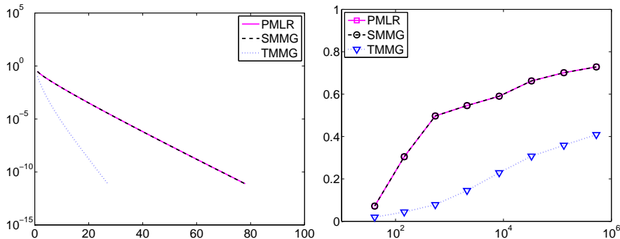
FIGURE 8. Spiral problem: Iteration history for nested iteration (left) and asymptotic convergence rates (right)
