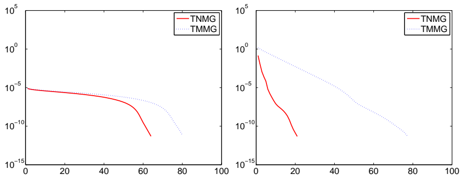
FIGURE 13. Degenerate Problem: Iteration histories for the initial iterates u_j^0 = \varphi_j (left) and u_j^0 = 0 > \varphi_j (right)
