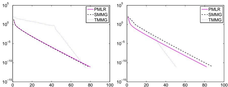
FIGURE 7. Spiral problem: Iteration histories for the initial iterates u_j^0 = \varphi_j (left) and u_j^0 = \varphi_j + 10 > \varphi_j (right)
