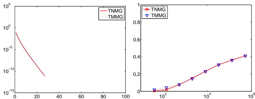
FIGURE 12. Spiral problem: Iteration history for nested iteration (left) and asymptotic convergence rates (right)
