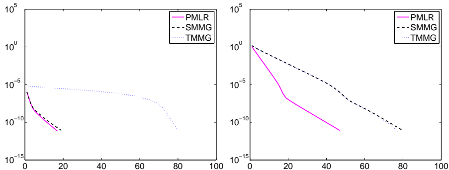
FIGURE 9. Degenerate Problem: Iteration histories for the initial iterates u_j^0 = \varphi_j (left) and u_j^0 = 0 > \varphi_j (right)
