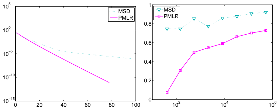
FIGURE 4. Spiral problem: Iteration history for nested iteration (left) and asymptotic convergence rates (right)
