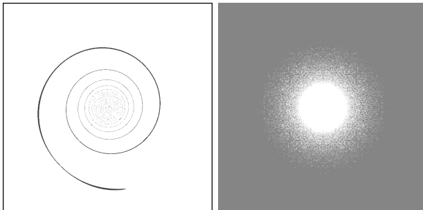
FIGURE 2. Coincidence sets of spiral problem (left) and degenerate problem (right)
