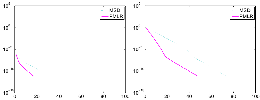
FIGURE 5. Degenerate problem: Iteration histories for the initial iterates u_j^0 = \varphi_j (left) and u_j^0 = \varphi_j + 10 > \varphi_j (right)
