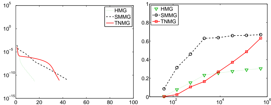
FIGURE 15. Degenerate Problem: Iteration history for nested iteration (left) and asymptotic convergence rates (right)
