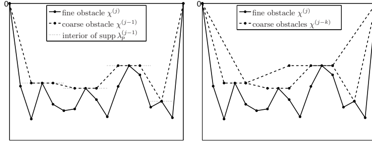
FIGURE 1. Restriction (left) and hierarchical decomposition (right) of defect obstacle
