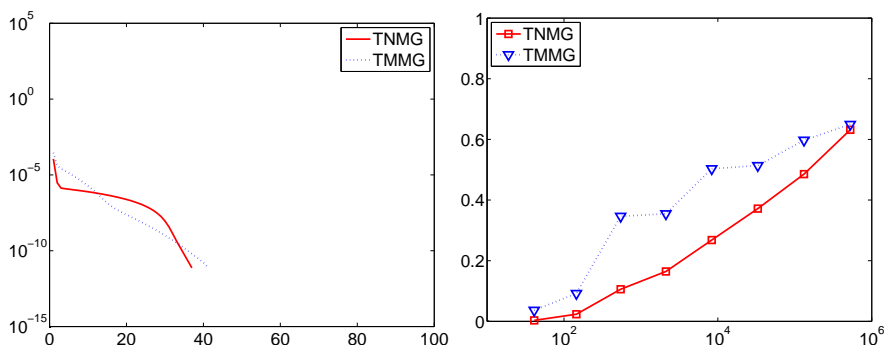
FIGURE 14. Degenerate Problem: Iteration history for nested iteration (left) and asymptotic convergence rates (right)
