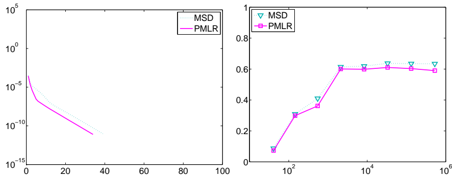
FIGURE 6. Degenerate problem: Iteration history for nested iteration (left) and asymptotic convergence rates (right)
