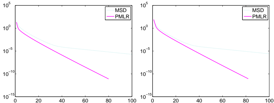
FIGURE 3. Spiral problem: Iteration histories for the initial iterates u_j^0 = \varphi_j (left) and u_j^0 = \varphi_j + 10 > \varphi_j (right)
