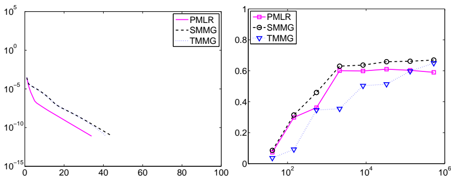
FIGURE 10. Degenerate Problem: Iteration history for nested iteration (left) and asymptotic convergence rates (right)
