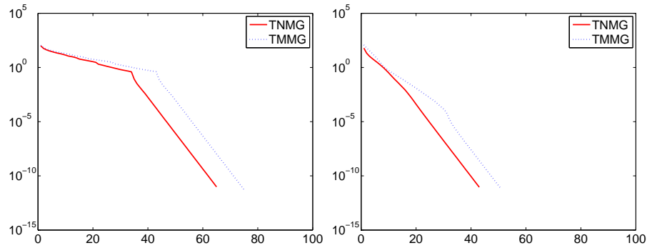
FIGURE 11. Spiral problem: Iteration histories for the initial iterates u_j^0 = \varphi_j (left) and u_j^0 = 0 > \varphi_j (right)
