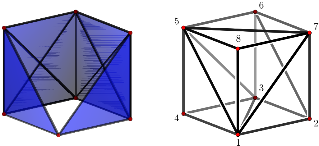
(a) The (3-dimensional) crosscut complex of some partial 3-cube C . The two quadrangle faces of C yield tetrahedra in \Gamma(C) , which are displayed almost flat.
