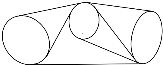
FIGURE 29. A pseudo-triangulation for three smooth convex obstacles.
