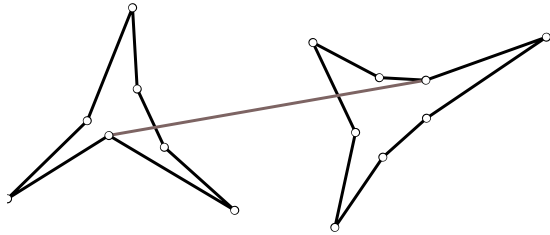
FIGURE 31. Two pseudo-triangles and their unique common tangent.
