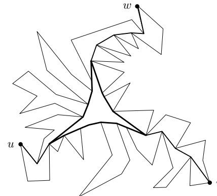
FIGURE 27. A geodesic triangle.
