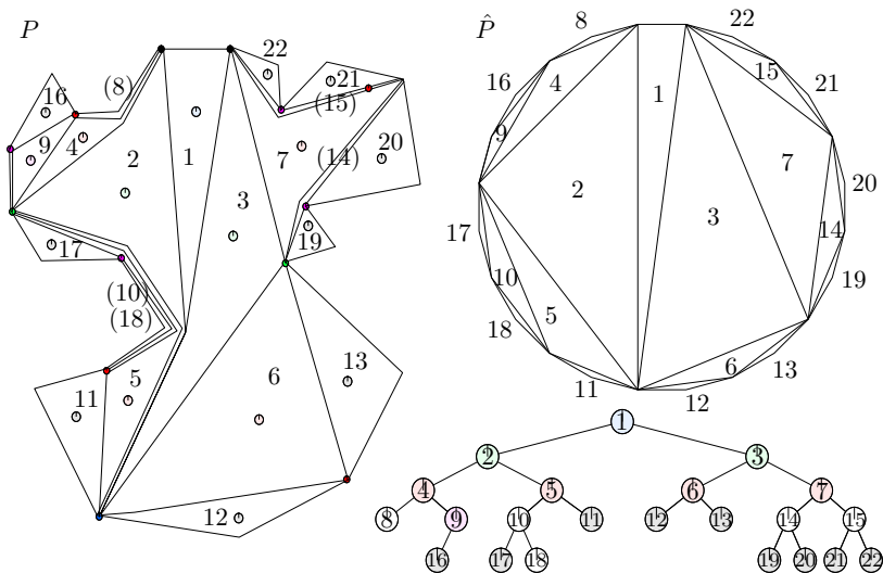
FIGURE 28. A geodesic triangulation of a polygon P , the corresponding triangulation \hat{T} of the convex polygon \hat{P} , and the binary tree representation. Some geodesic triangles in P have no area; their numbers are given in parentheses.
