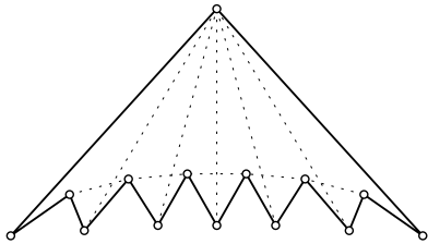
FIGURE 10. A pseudo- k -gon with 2^{k-3} pseudo-triangulations.
