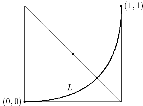
Figure 1: The limit shape L .
